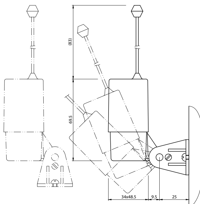
Positions for outdoor mounting.
